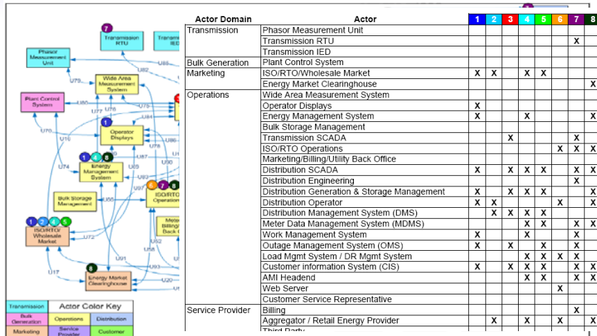
Unified Logical Interface Diagram* - Mapped to Key System Interfaces for Integrating Distributed Energy Resources * Unified Logical Interface Diagram from NISTIR 7628 - Smart Grid Cyber Security Strategy & Requirements, Feb. 2010
